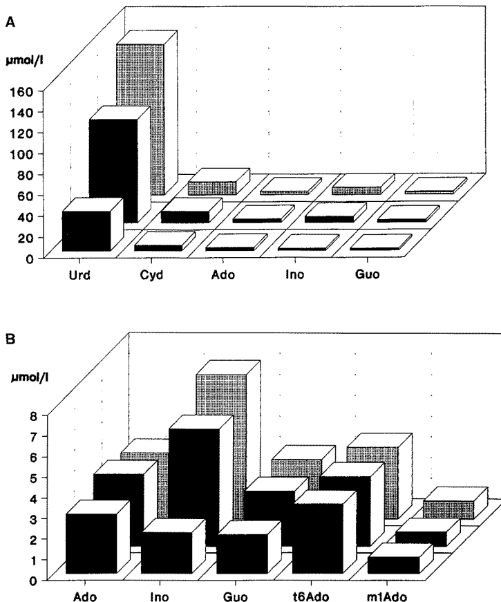
Fig. 3. Time-dependent alterations of the ribonucleoside concentrations due to postsecretory activities in colostral bovine milk: acidic preservation of the milk samples was carried out at 0 min (■), 30 min (▨), and 60 min (□) after milking. A: unmodified ribonucleosides; B: modified ribonucleosides in comparison to unmodified purine ribonucleosides.
