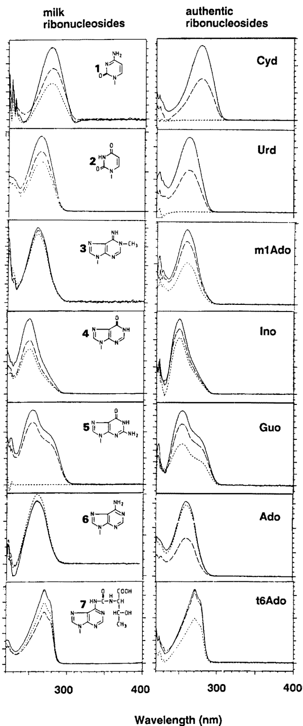
Fig. 1b. UV-spectra of the ribonucleosides (peak maximum (—), up-slope (....), down-slope (---): peaks 1–7 analyzed by HPLC of 100 \mu l of bovine colostrum milk compared with authentic ribonucleosides showing isochromatographic behavior (compare “Materials and methods”).
